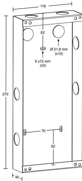
Flush mount back box
